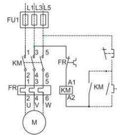
Wiring Diagram
